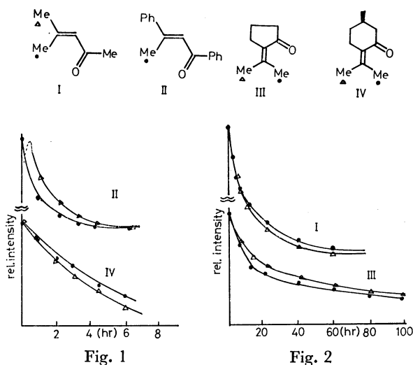
Fig. 1 and 2. Decrease of NMR signal-intensities of \alpha -methyls versus irradiation period.
